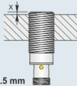
Flush mounting
