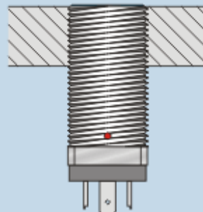
Flush mounting
