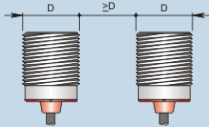
Side by side mounting
