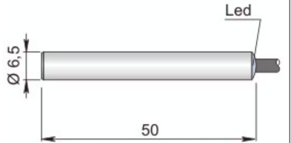
Dimension in mm
