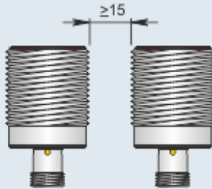
Side by side mounting
