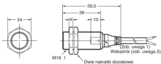
E2A-M18KS08-WP-□□/E2A-S18KS08-WP-□
