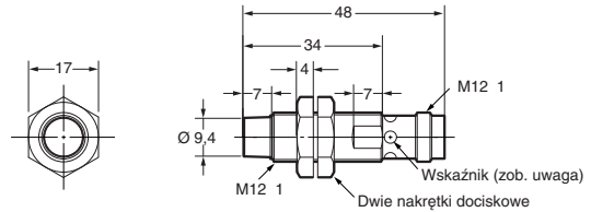
E2A-M12KN08-M1-□□/E2A-S12KN08-M1-□
