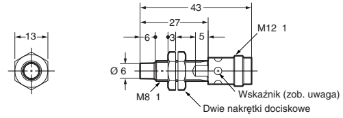
E2A-S08KN04-M1-□□
