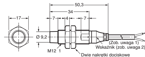
E2A-M12KN08-WP-□□/E2A-S12KN08-WP-□
