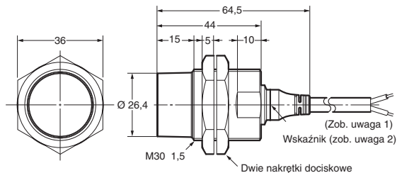
E2A-M30KN20-WP-□□/E2A-S30KN20-WP-□
