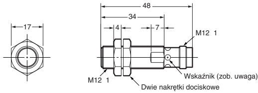
E2A-M12KS04-M1-□□/E2A-S12KS04-M1-□
