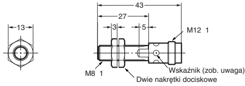
E2A-S08KS02-M1-□□
