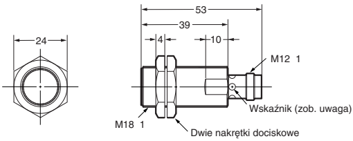
E2A-M18KS08-M1-□□/E2A-S18KS08-M1-□
