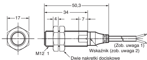
E2A-M12KS04-WP-□□/E2A-S12KS04-WP-□
