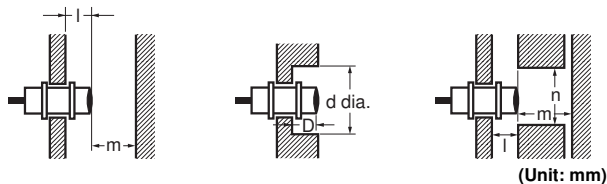
Double Sensing Distance Type <Shielded>
