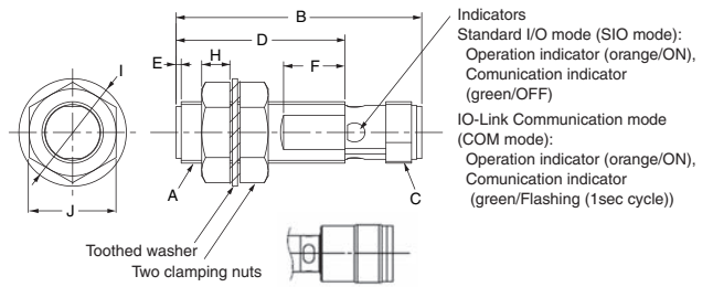
Model E2EQ-X□8-M1; Shape of connection.
