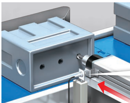
Spindle presence detection
