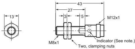
E2A-S08KS02-M1-□□
