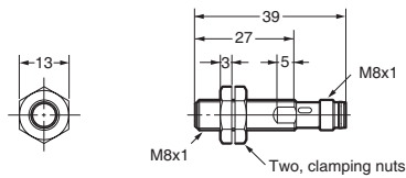
E2A-S08KS02-M5-□□/E2A-S08KS02-M3-□
