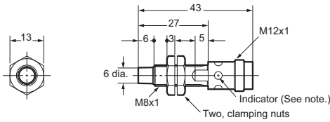
E2A-S08KN04-M1-□□
