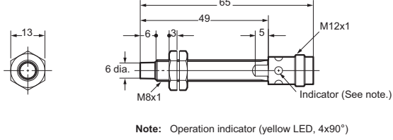
E2A-S08LN04-M1-□□
