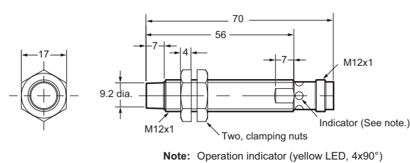
E2A-S12LN08-M1-□
