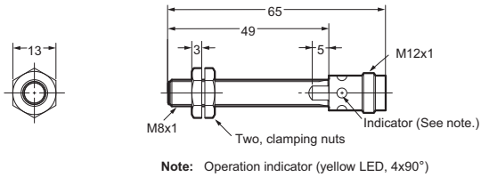
E2A-S08LS02-M1-□□
