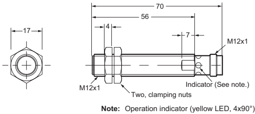
E2A-S12LS04-M1-□
