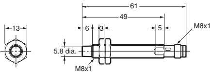
E2A-S08LN04-M5-□□/E2A-S08LN04-M3-□
