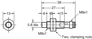
E2A-S08KN04-M5-□□/E2A-S08KN04-M3-□
