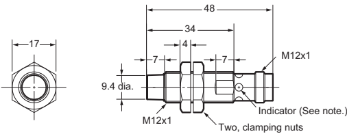
E2A-S12KN08-M1-□
