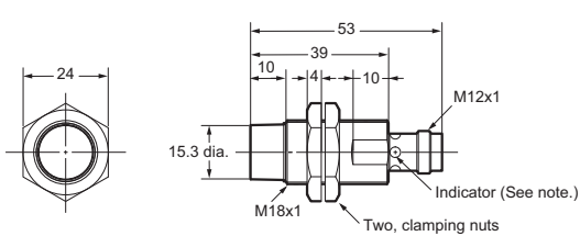
E2A-S18KN16-M1-□
