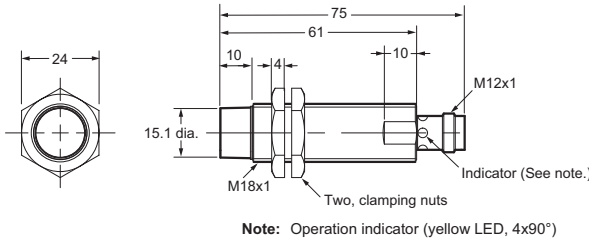
E2A-S18LN16-M1-□
