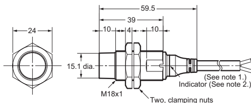
E2A-S18KN16-WP-
