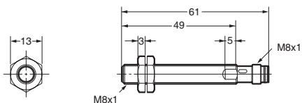
E2A-S08LS02-M5-□□/E2A-S08LS02-M3-□
