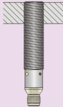
Flush mounting
