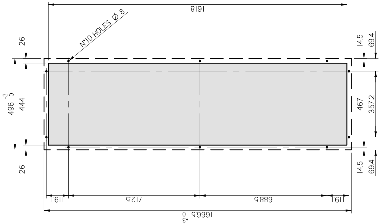
MONTAGGIO A INCASSO / SEMINCASSO FLUSH / SEMI-FLUSH MOUNTING
