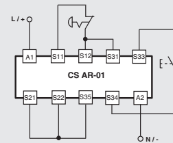
Input configuration with manual start 1 channel
