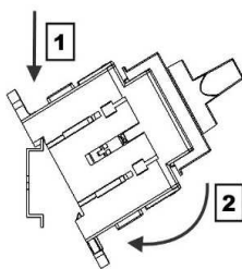
Montagebild (T) Mounting image (T)
