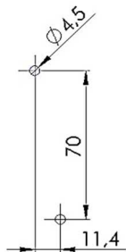
Bohrbild (V) Drilling pattern (V)
