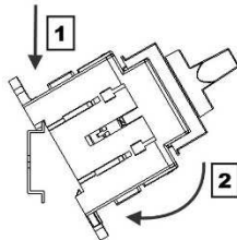
Montagebild (V) Mounting image (V)
