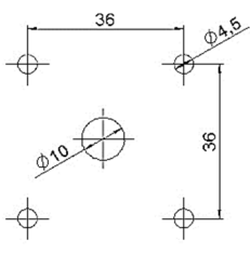
Bohrbild D0 (E) Drilling pattern D0 (E)
