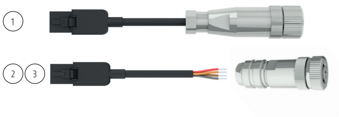
Photo: Fully assembled sensor cable with connector and female M12 plug, 2.0 m long (Art. No. 244445)
