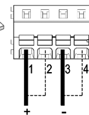
X1 Operating voltage connection
