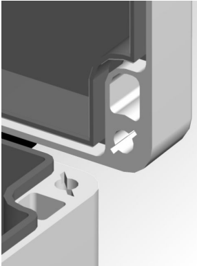
RFI Shielding (metalised spray coating to interior)
