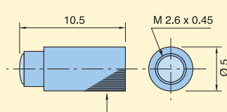
LENTE MOD. AT 4101 - ACF000006 LENS VIEWER AT 4101
