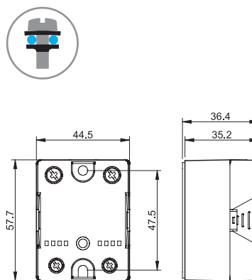
Type 77.x5 Screw terminal (plate clamp)
