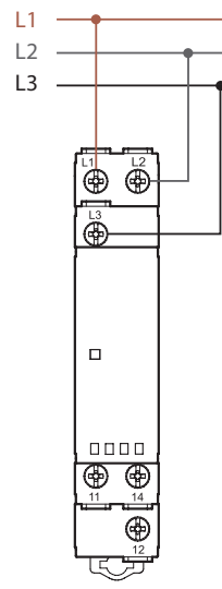
Type 70.61
