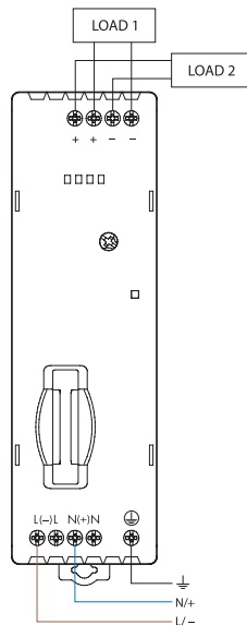
Wiring diagram for 78.2A
