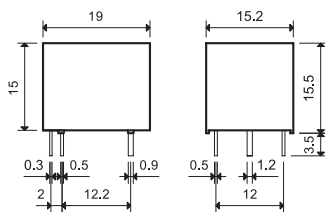
Type 36.11-4011
