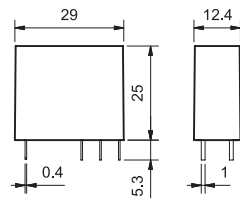
Types 40.31/51/52/61 (page 40)
