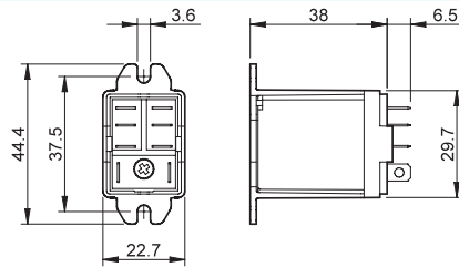
056.25 with relay
