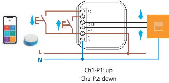
Type 13.52
