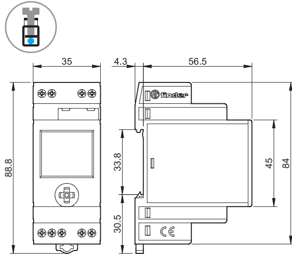
Type 11.91 Screw terminal
