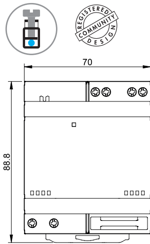
Types 78.51 / 78.61 Screw terminal
