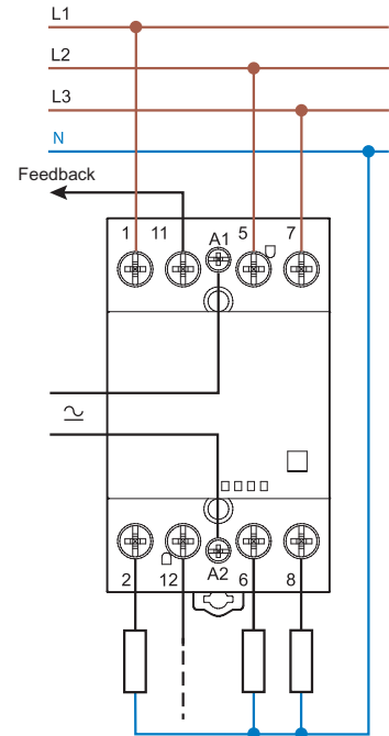
Type 22.xx.4717
