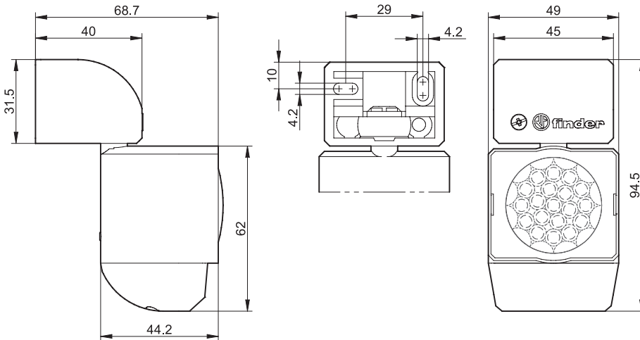
Type 18.11
