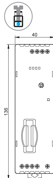
Type 78.1B Screw terminal
