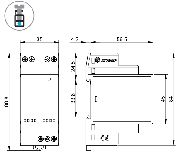
Types 78.50 / 78.60 Screw terminal
