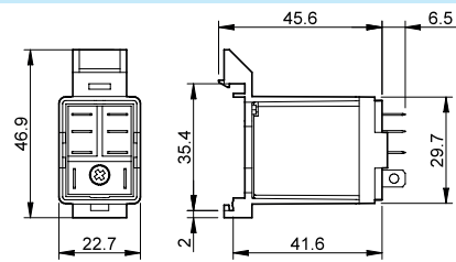
056.27 with relay
