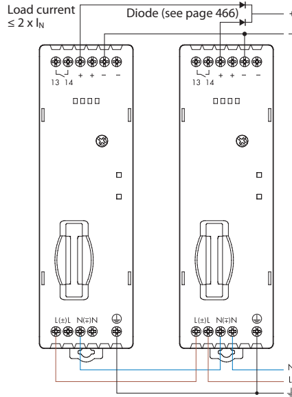
Parallel connection
