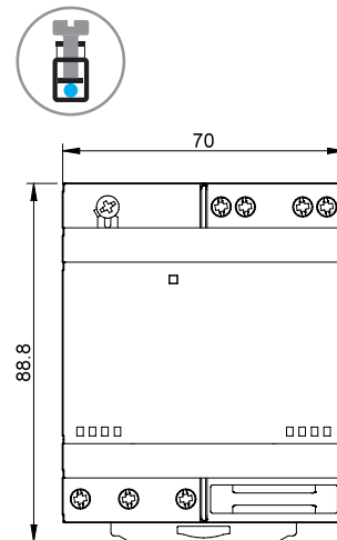
Type 78.1B Screw terminal
