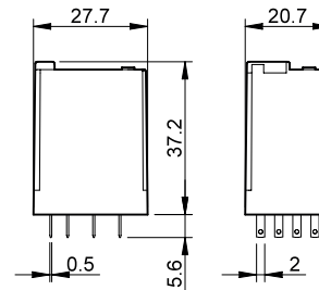
Type 55.34
