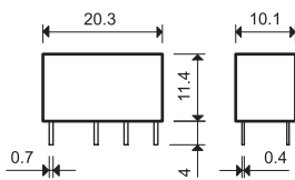
Type 30.22
