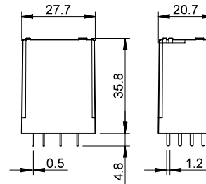
Type 55.14
