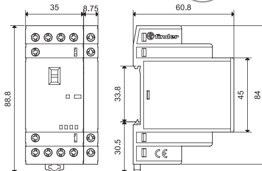
Types 22.44/22.64 + 022.63/022.65 Screw terminal
