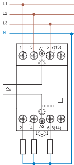
Type 22.44/22.64
