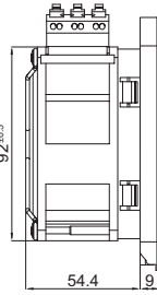
AC version
