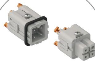
CKSH SQUICH® 10A SPRING contacts with actuator
