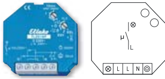
Typical connection
