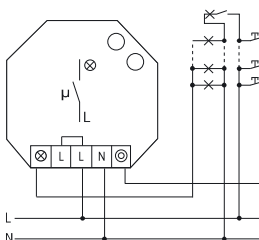
4-wire circuit with attic lighting, resettable
