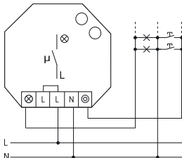
3-wire circuit, resettable
